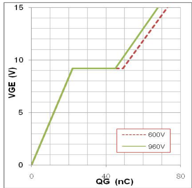
Figure18:typical gate charge VS. VGE,IC=15A
