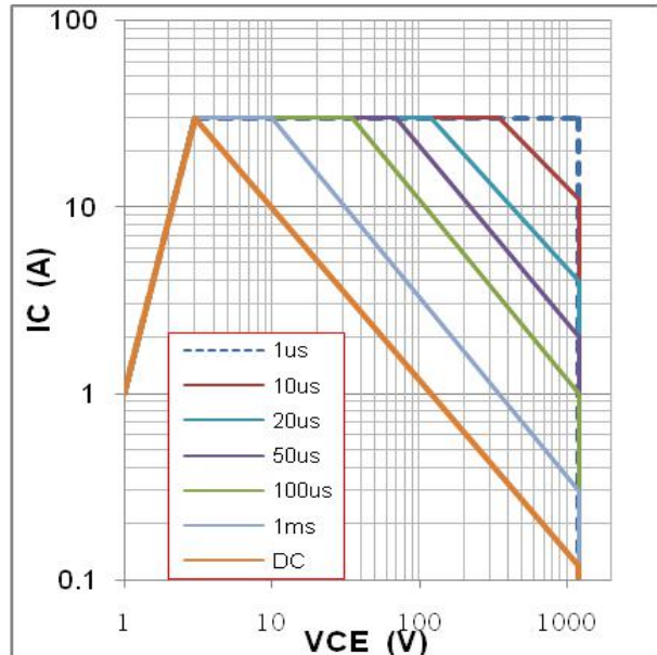
Figure4:forward SOA,TC=25°C,TJ≤150°C
